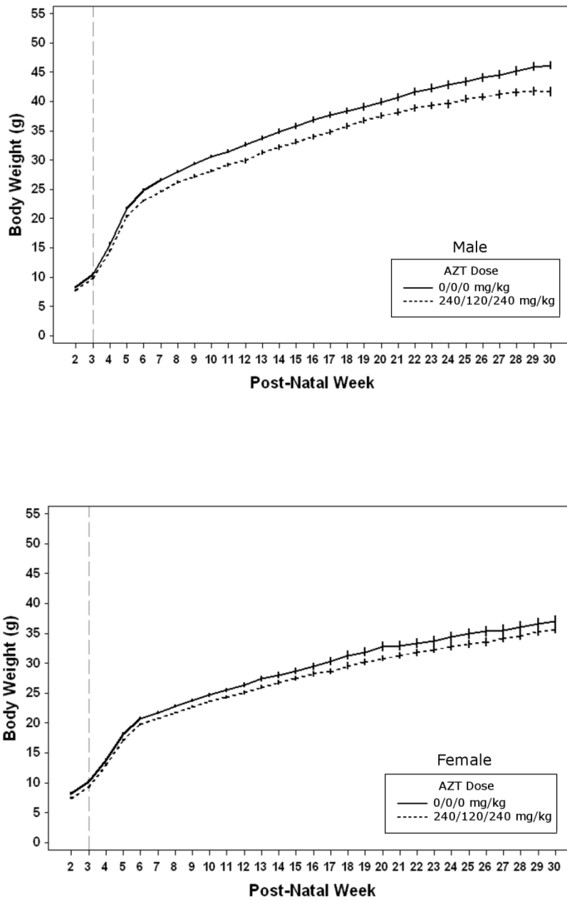
FIGURE 4 Growth Curves for Mice Administered AZT by Gavage in the 30-Week In Utero /Postnatal Study of AZT
