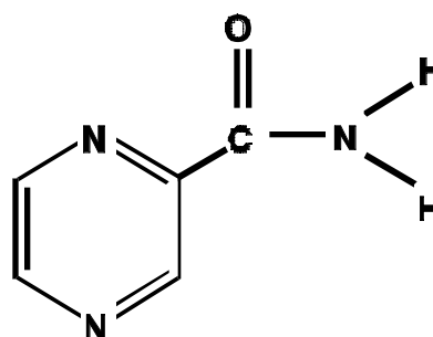
Pyrazinamide Molecular Formula: C_5H_5N_3O Molecular Weight: 123.12 CAS No.: 98-96-4
