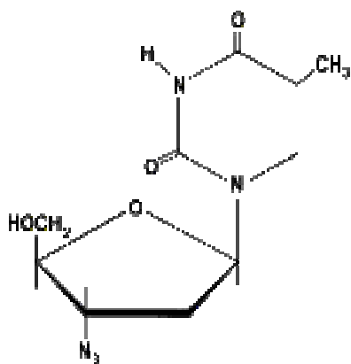
AZT Molecular Formula: C_{10}H_{13}N_5O_4 Molecular Weight: 267.24 CAS No.: 30516-87-1
