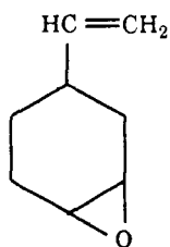
4 -Vinyl-1,2-epoxycyclohexane (4 -Vinylcyclohexene monoxide, 4 -Vinylcyclohexene-1,2-epoxide)
