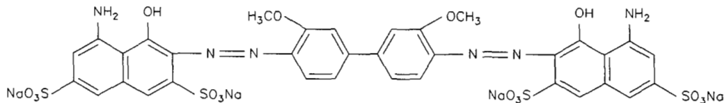
C.I. Direct Blue 15 CAS No. 2429-74-5
