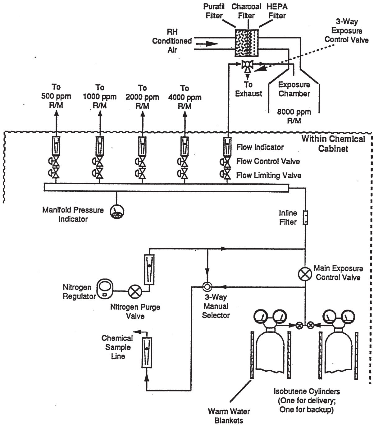
FIGURE J3 Schematic of Generation and Delivery System
