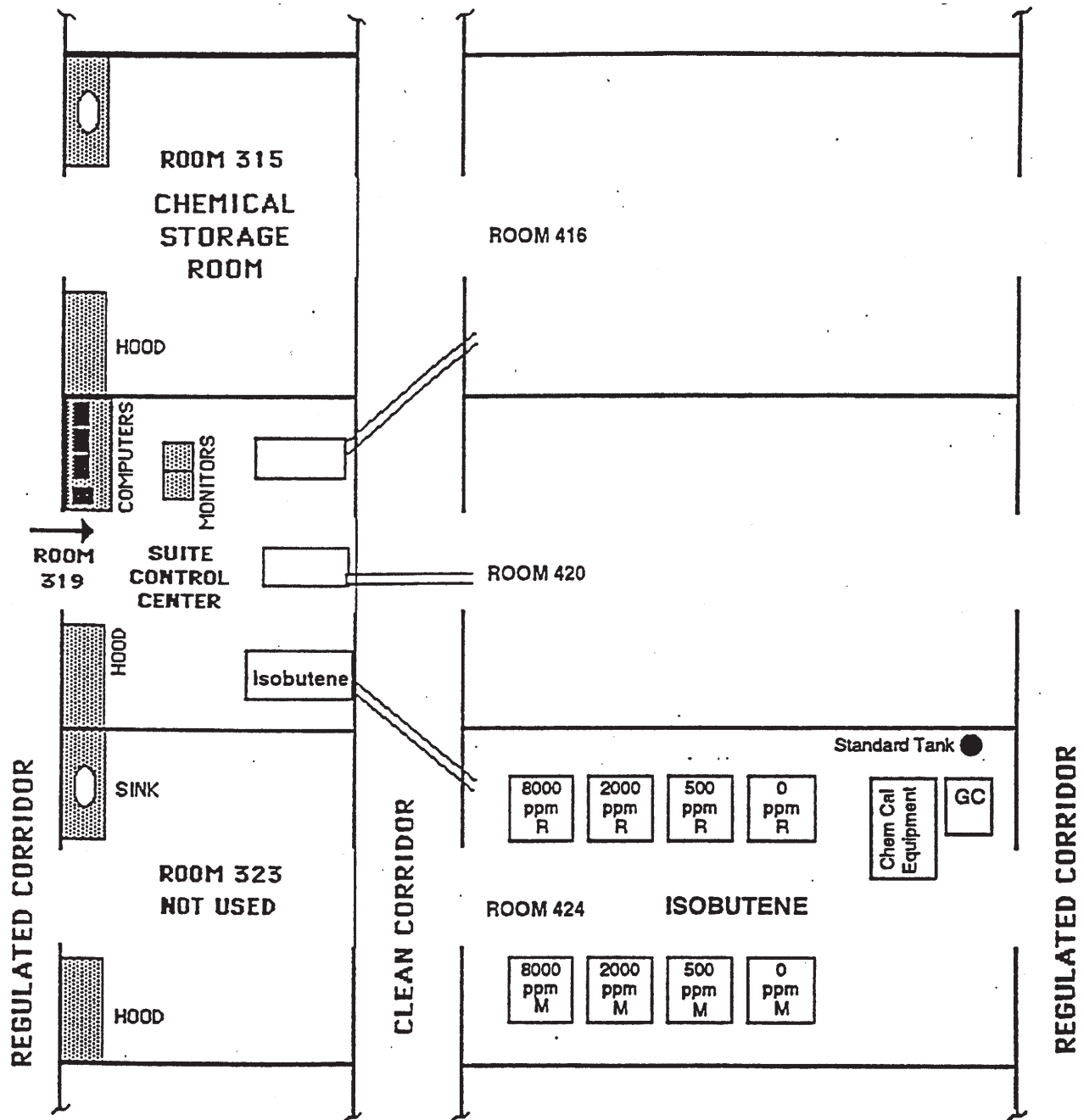
FIGURE J5 2 Year Inhalation Suite
