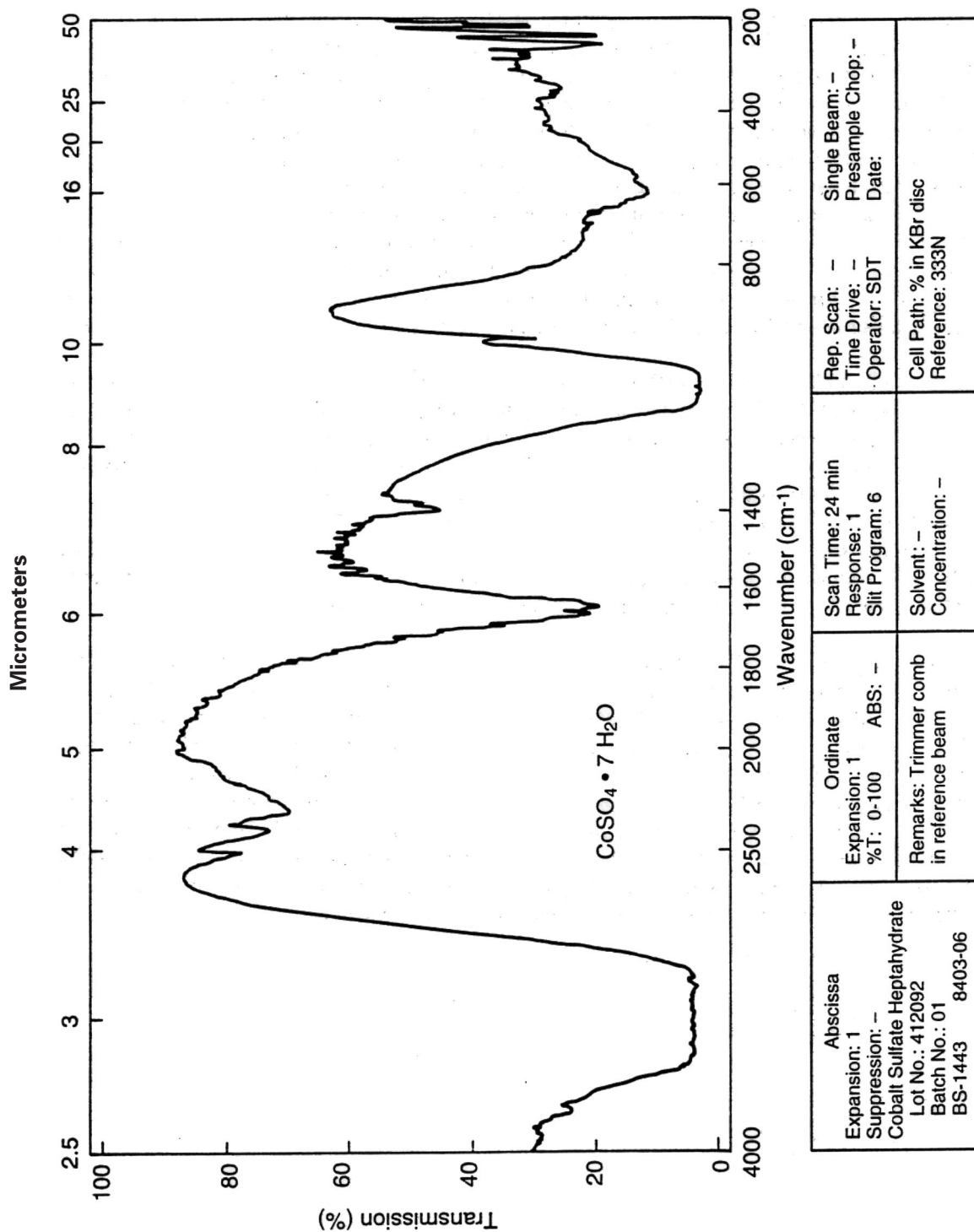
FIGURE F1 Infrared Absorption Spectrum of Cobalt Sulfate Heptahydrate
