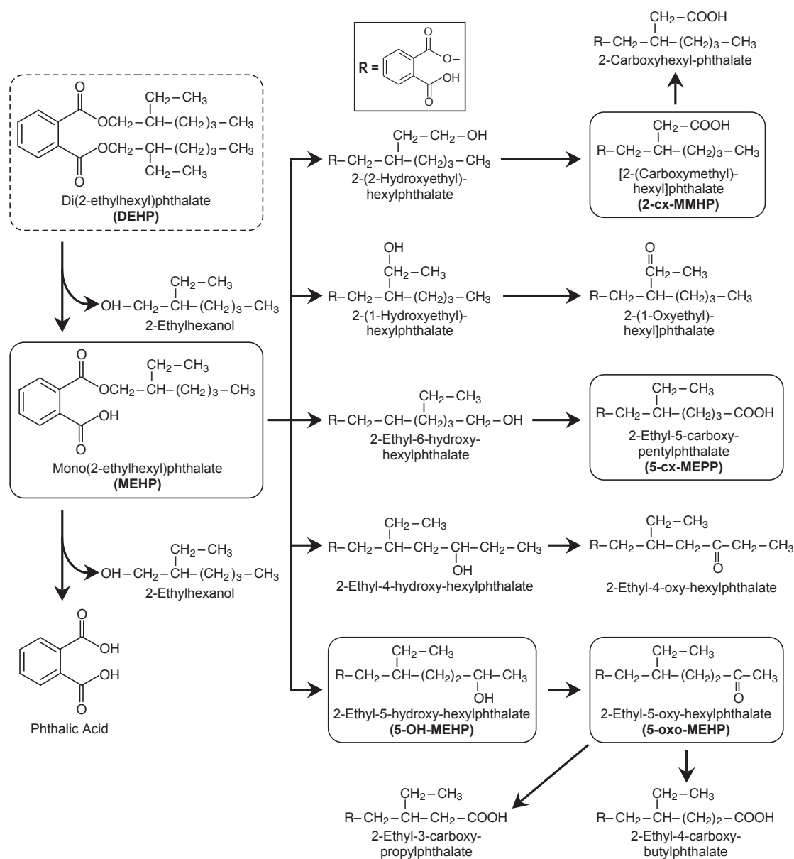
Figure 5. DEHP Metabolism
