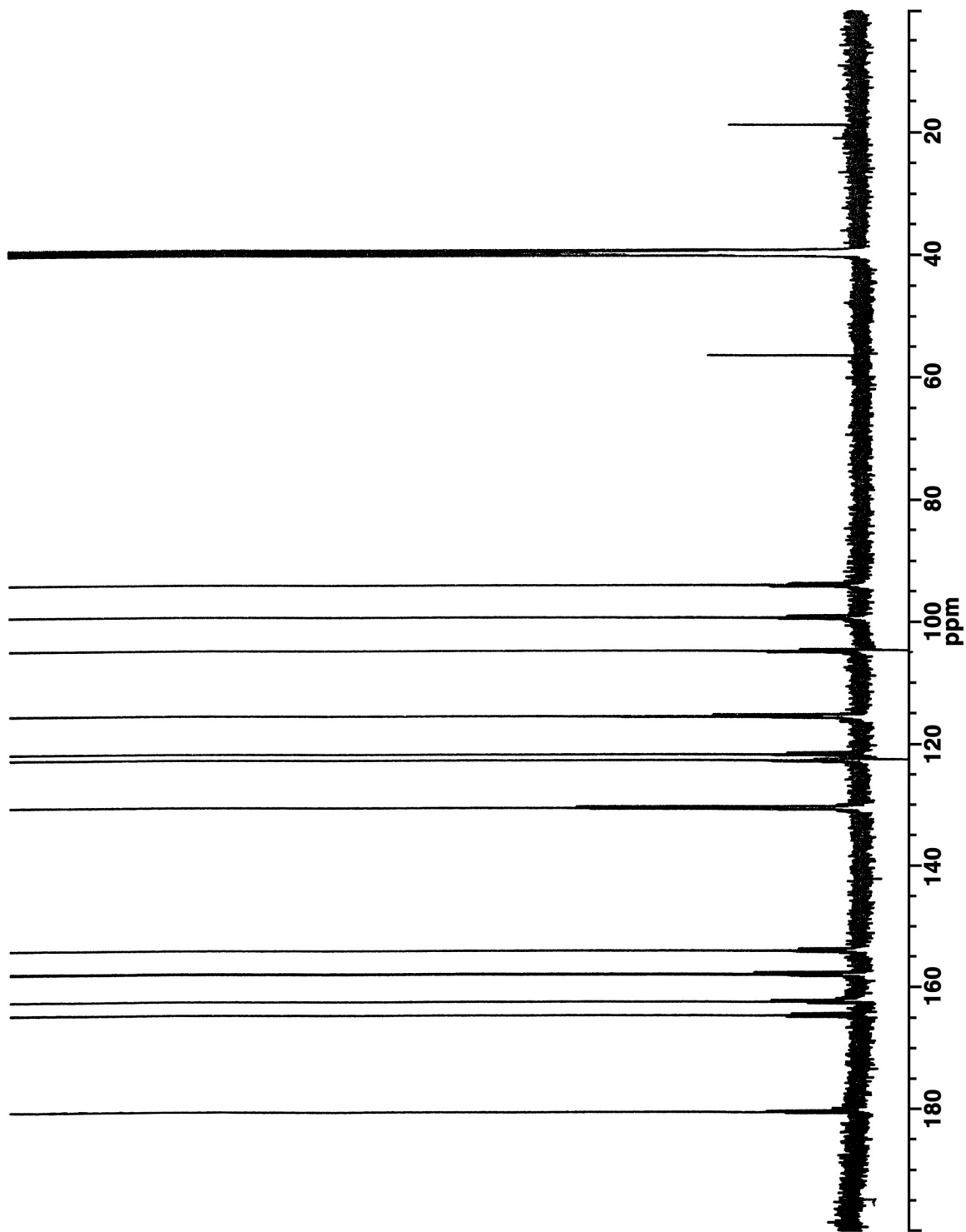
FIGURE A3 13 C-Nuclear Magnetic Resonance Spectrum of Genistein
