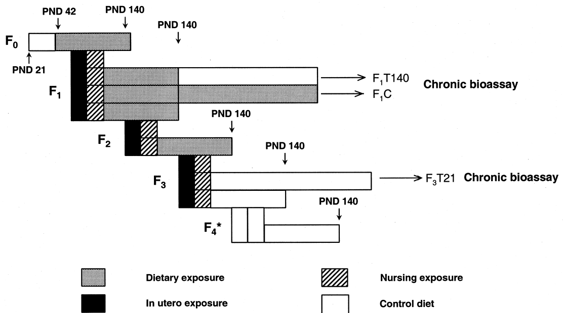
FIGURE 1 Dosing Schedule for the Multigenerational Reproductive Toxicology and Chronic Studies * The F 4 generation was mated similarly to generations F 0 to F 3 to produce the F 5 generation
