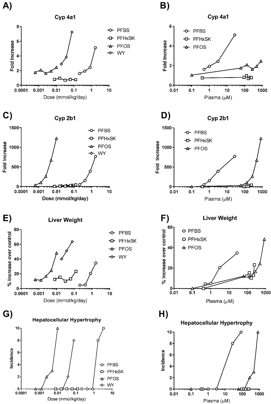
Figure 30. Average Magnitude of Change for Cyp4a1 Expression (A, B), Cyp2b1 Expression (C, D), Liver Weight Increase (E, F), and Hepatocellular Hypertrophy (G, H) in Female Sprague Dawley Rats Administered Perfluorobutane Sulfonic Acid, Perfluorohexane Sulfonate Potassium Salt, or Perfluorooctane Sulfonic Acid
