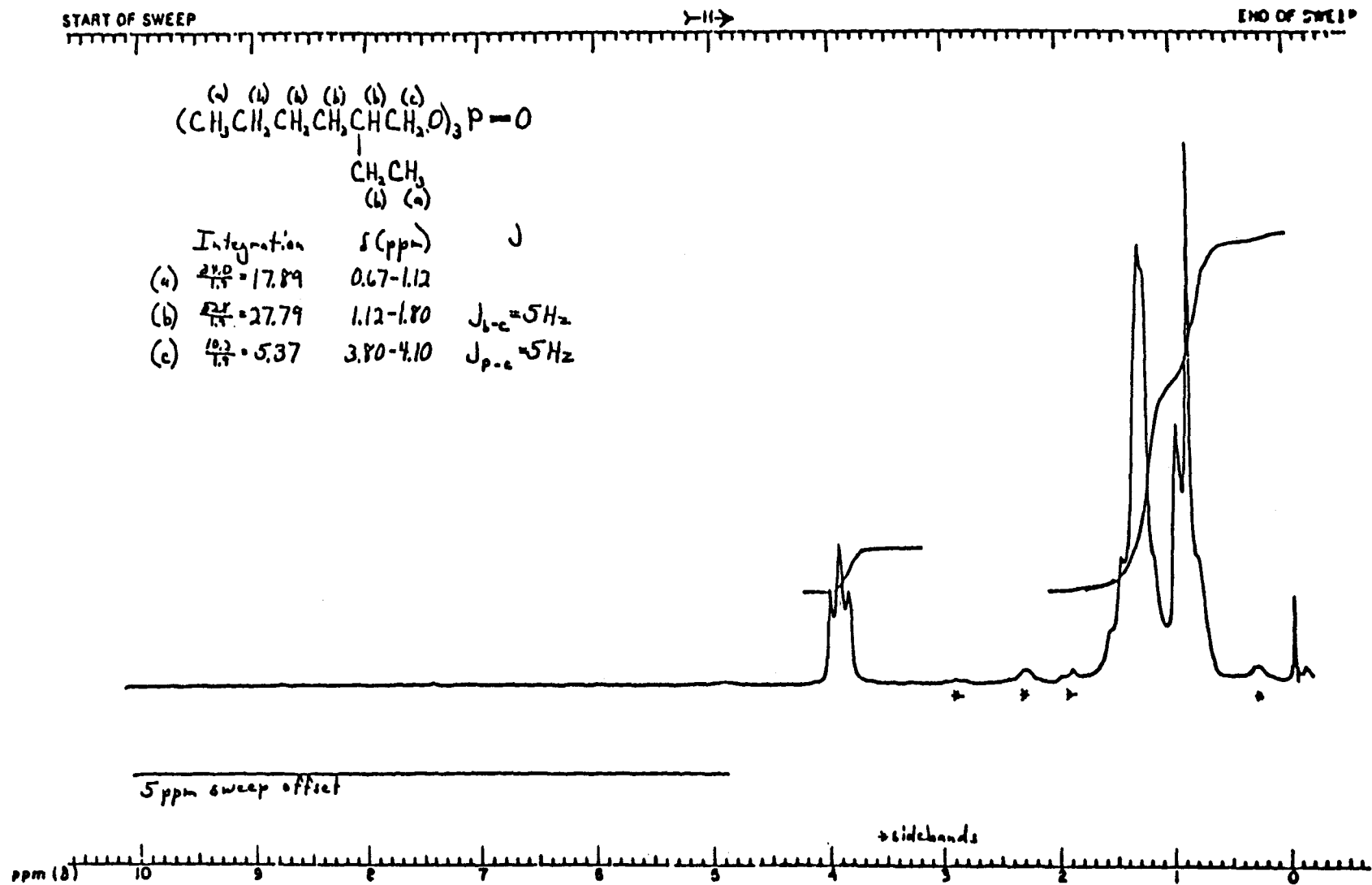
FIGURE 8. NUCLEAR MAGNETIC RESONANCE SPECTRUM OF TRIS(2-ETHYLHEXYL)PHOSPHATE (LOT NO. TP121580)
