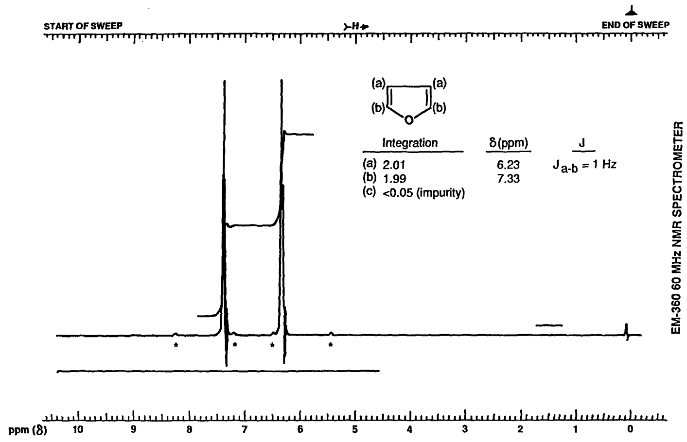
FIGURE H2 Nuclear Magnetic Resonance Spectrum of Furan
