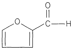
Furfural
