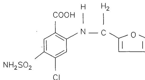
Furosemide
