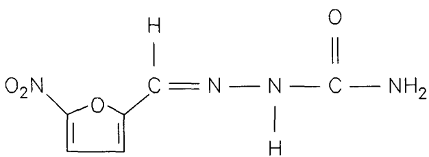
Nitrofurazone
