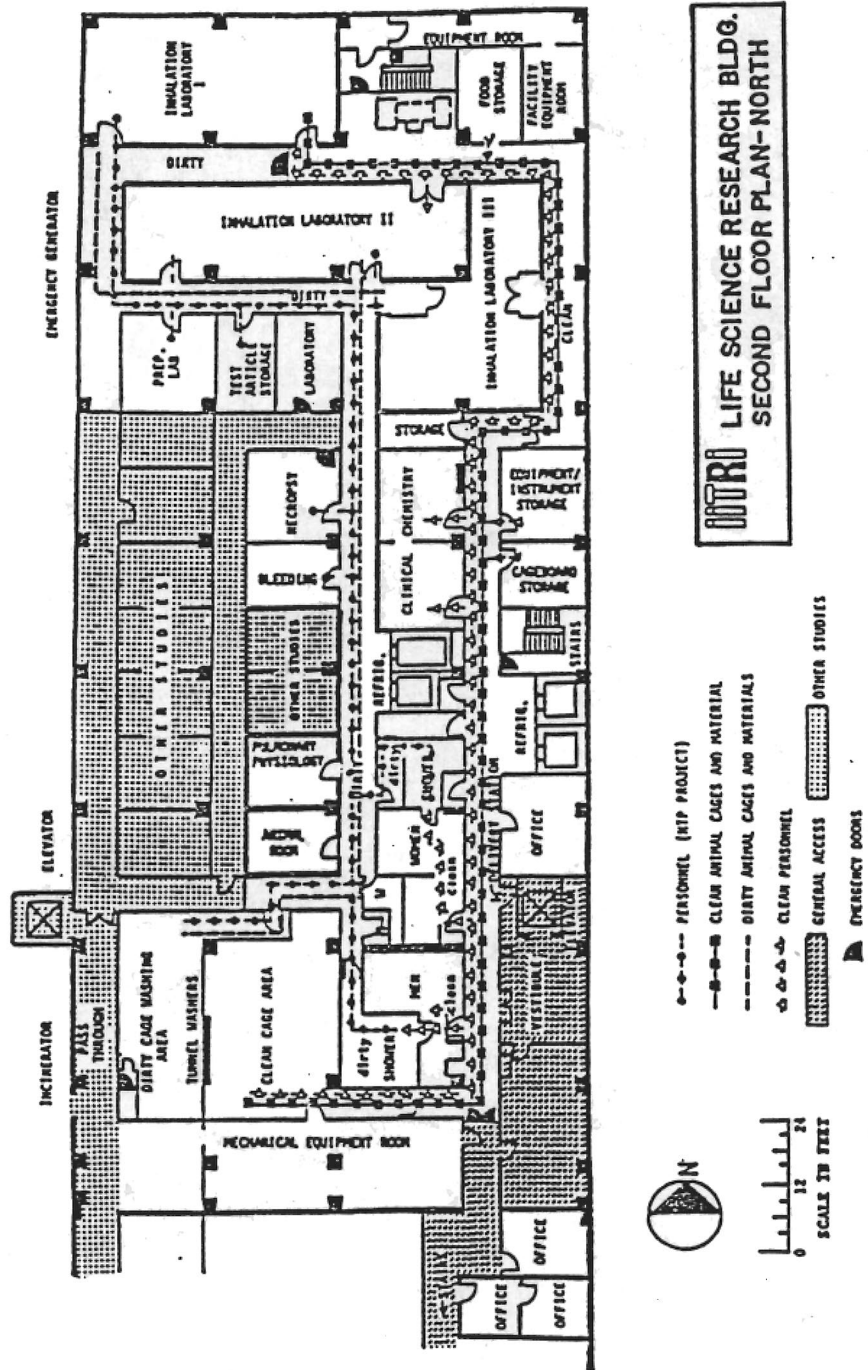
FIGURE F4 Inhalation Suite
