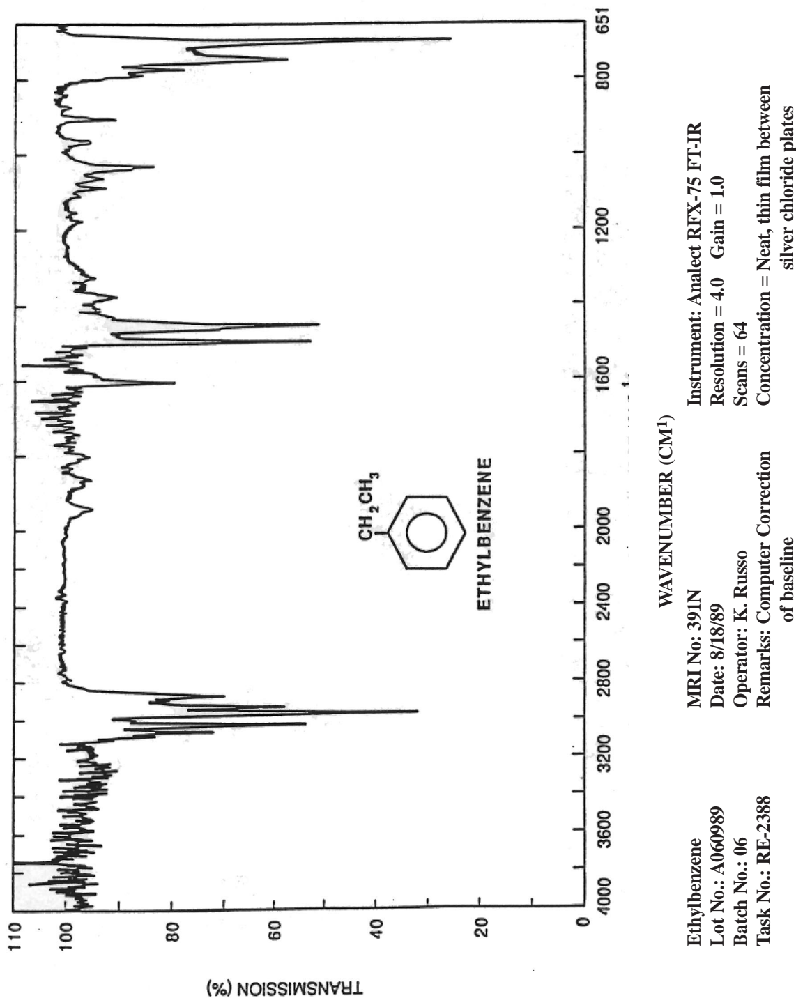
FIGURE F1 Infrared Absorption Spectrum of Ethylbenzene
