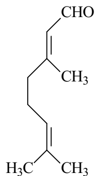
Geranial
