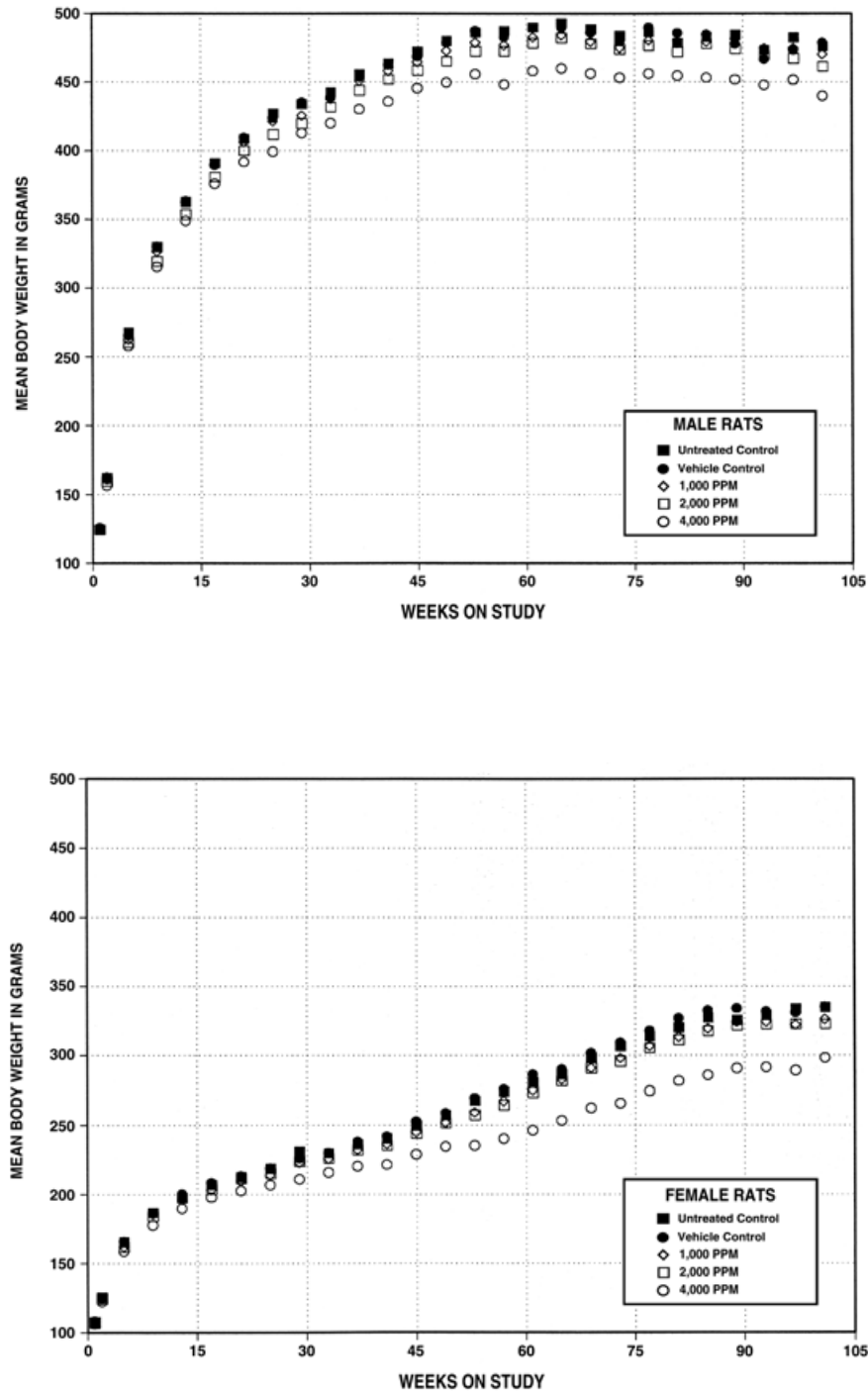
FIGURE 3 Growth Curves for Male and Female Rats Exposed to Citral in Feed for 2 Years
