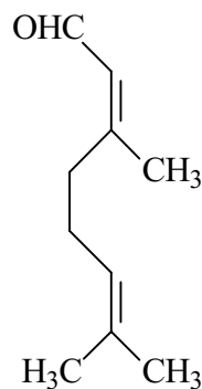
Neral
