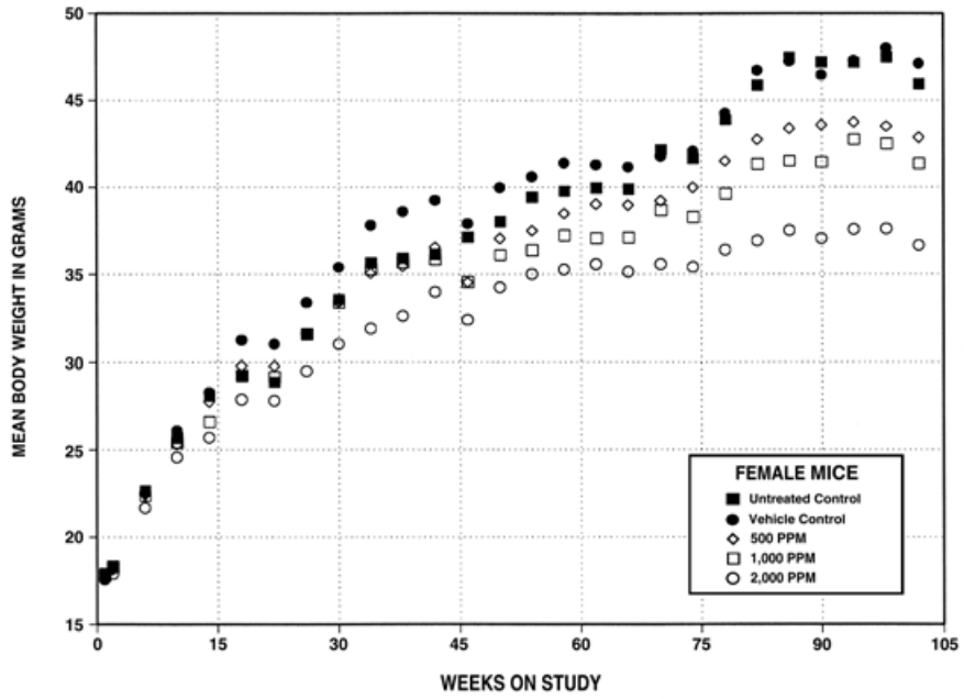
FIGURE 5 Growth Curves for Male and Female Mice Exposed to Citral in Feed for 2 Years
