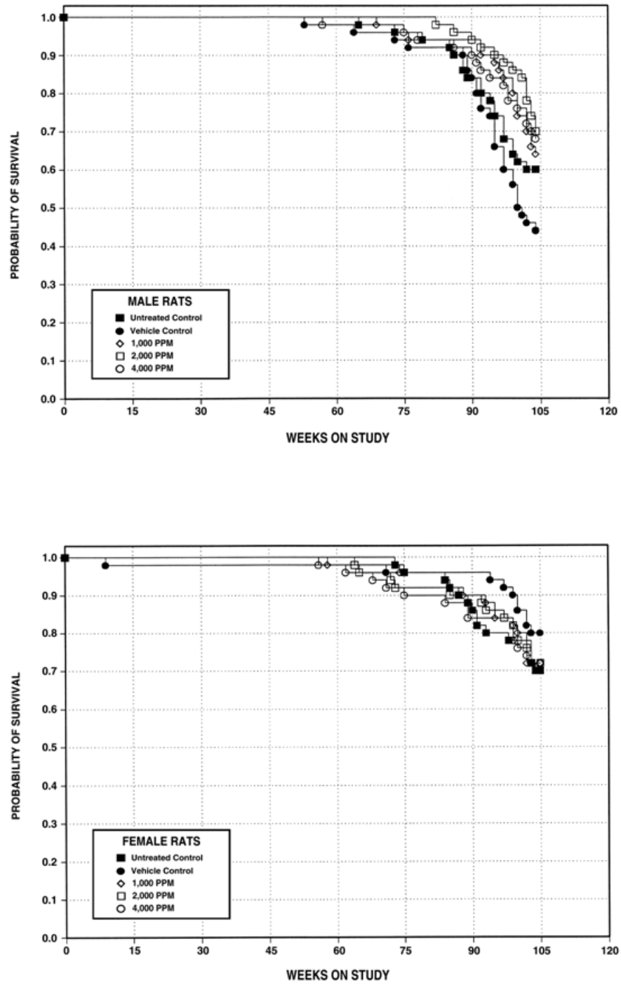
FIGURE 2 Kaplan-Meier Survival Curves for Male and Female Rats Exposed to Citral in Feed for 2 Years
