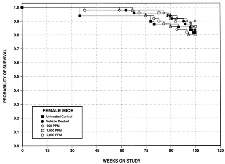
FIGURE 4 Kaplan-Meier Survival Curves for Male and Female Mice Exposed to Citral in Feed for 2 Years
