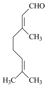
Geranial
