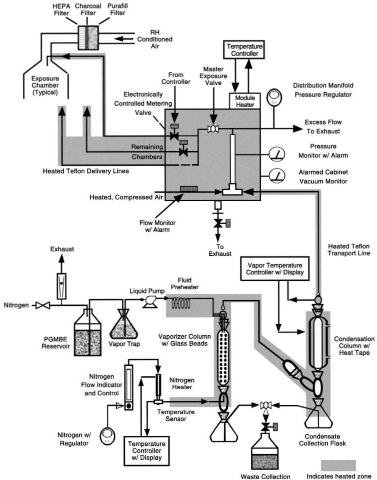
FIGURE K5 Schematic of the Vapor Generation and Delivery System in the Inhalation Studies of Propylene Glycol Mono- t -butyl Ether
