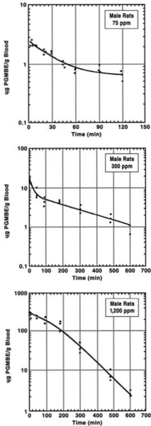
FIGURE N1 Blood Concentrations of Propylene Glycol Mono- t -butyl Ether in Male F344/N Rats after a Single 6-Hour Exposure to Propylene Glycol Mono- t -butyl Ether by Inhalation
