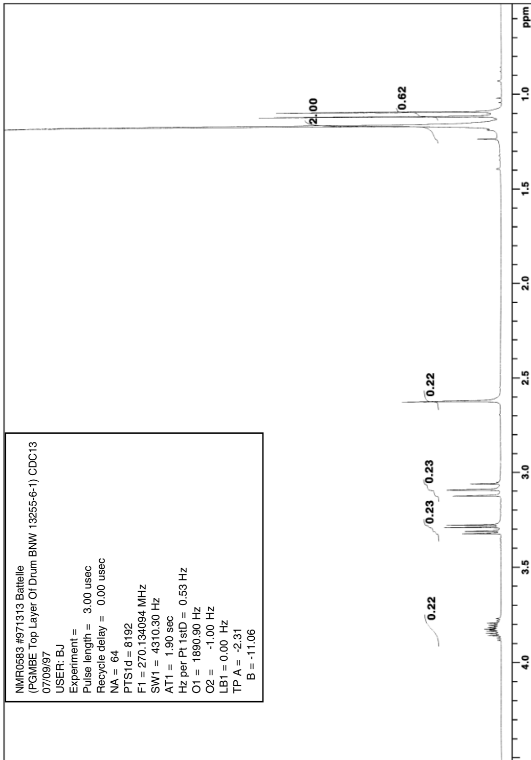
FIGURE K2 1 H-Nuclear Magnetic Resonance Spectrum of Propylene Glycol Mono- t -butyl Ether
