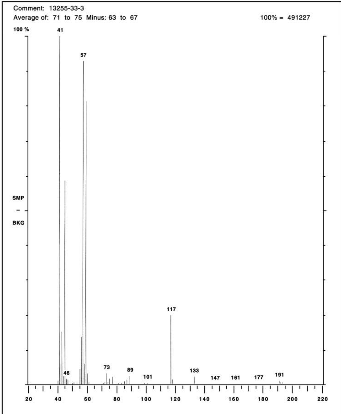
FIGURE K4 Mass Spectrum of Propylene Glycol Mono- t -butyl Ether
