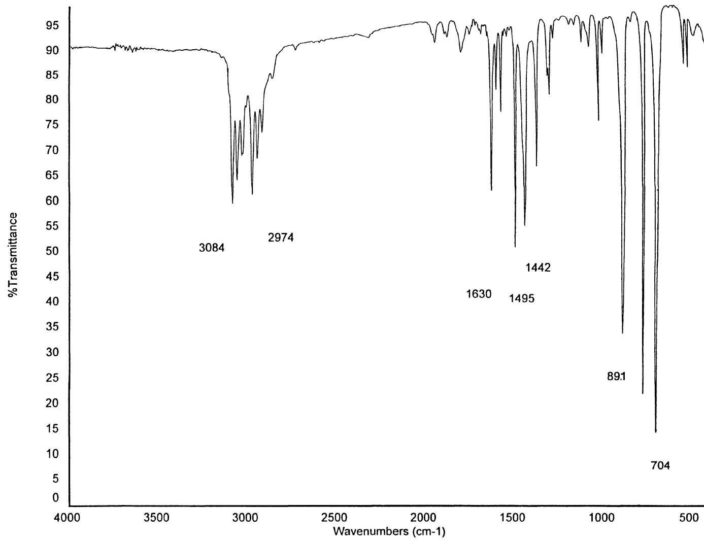
FIGURE II Infrared Absorption Spectrum of \alpha -Methylstyrene, Lot BNW 13871-4
