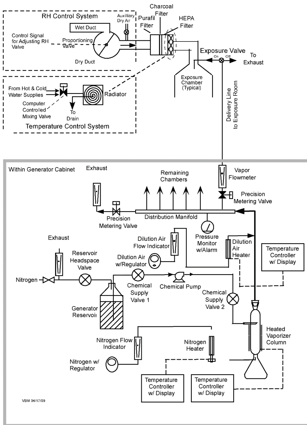
FIGURE H4 Schematic of the Vapor Generation and Delivery System in the 2-Year Inhalation Studies of 2,3-Butanedione
