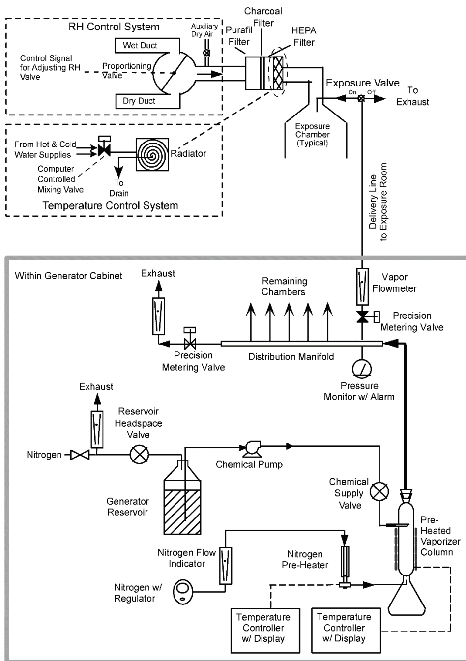
FIGURE H3 Schematic of the Vapor Generation and Delivery System in the 3-Month Inhalation Studies of 2,3-Butanedione
