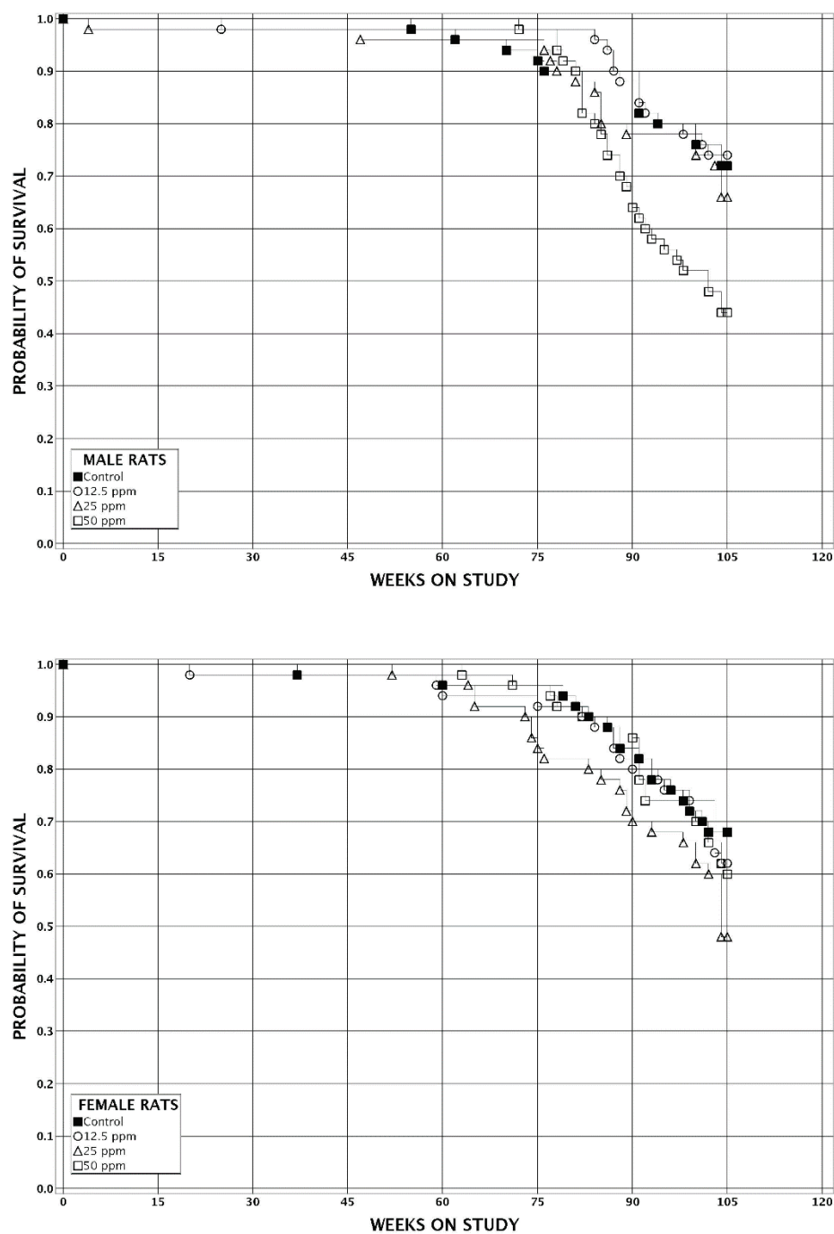
FIGURE 2 Kaplan-Meier Survival Curves for Rats Exposed to 2,3-Butanedione by Inhalation for 2 Years
