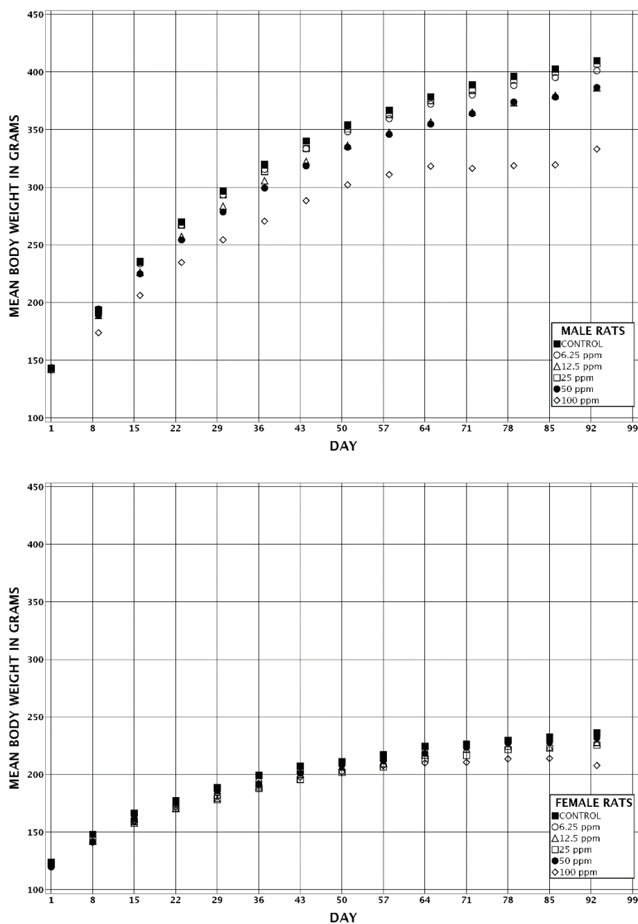
FIGURE 1 Growth Curves for Rats Exposed to 2,3-Butanedione by Inhalation for 3 Months
