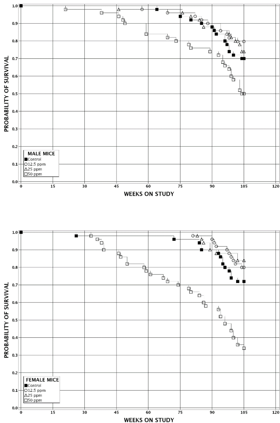
FIGURE 5 Kaplan-Meier Survival Curves for Mice Exposed to 2,3-Butanedione by Inhalation for 2 Years
