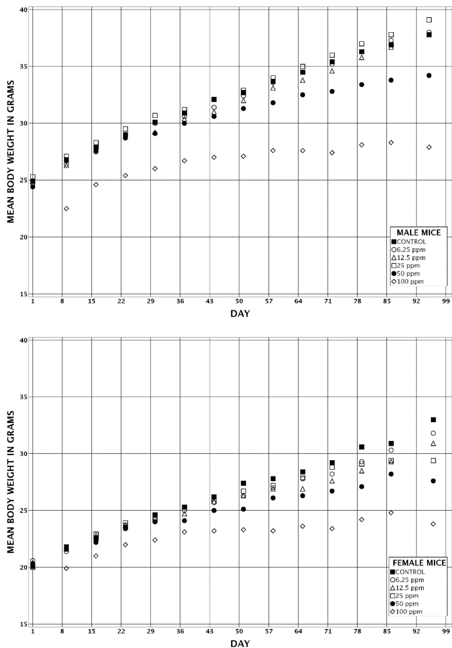
FIGURE 4 Growth Curves for Mice Exposed to 2,3-Butanedione by Inhalation for 3 Months
