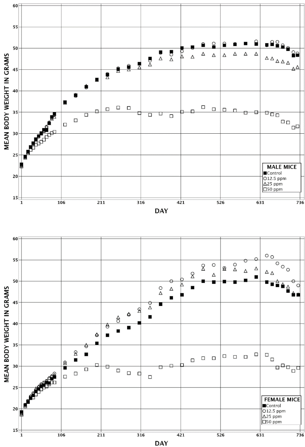
FIGURE 6 Growth Curves for Mice Exposed to 2,3-Butanedione by Inhalation for 2 Years
