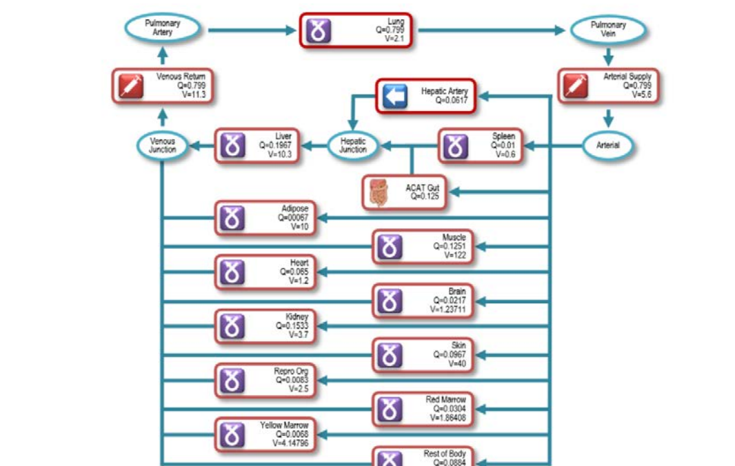
Figure 2. Structure of the GastroPlus Rat PBPK Model
