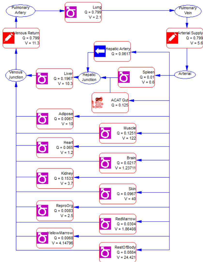
Figure 2 Structure of the GastroPlus Rat PBPK Model
