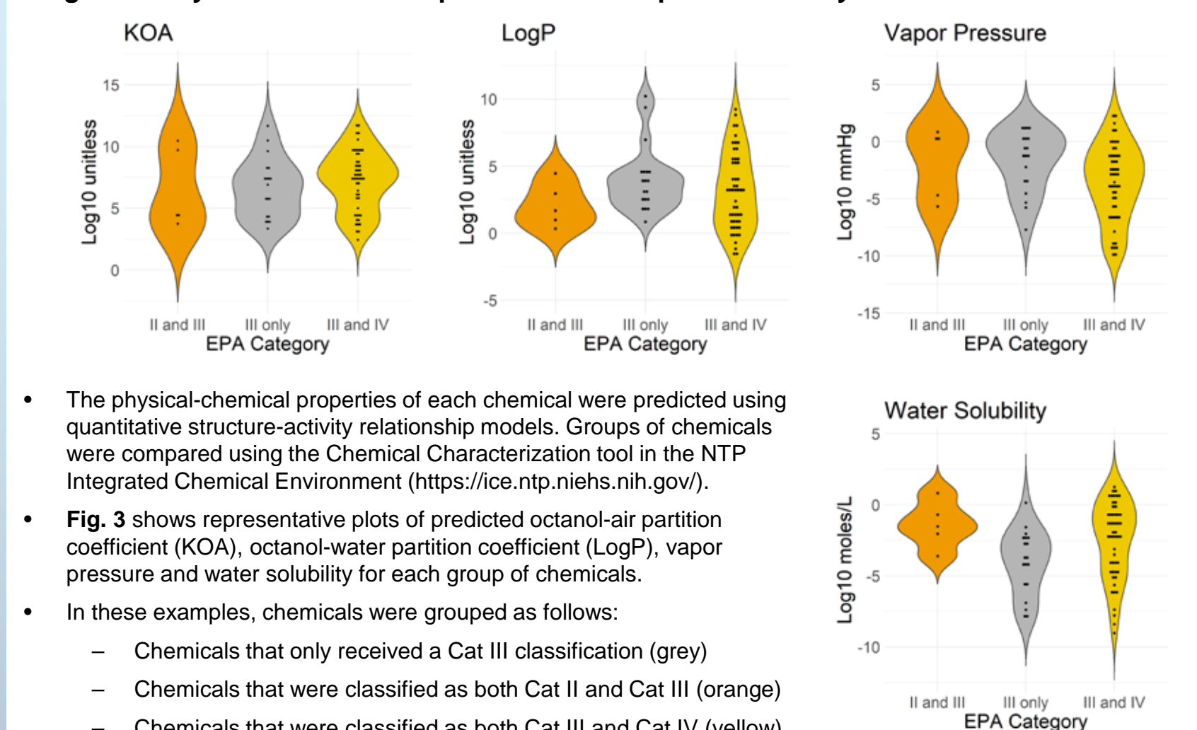
Figure 3: Physical-chemical Properties Do Not Explain Variability
