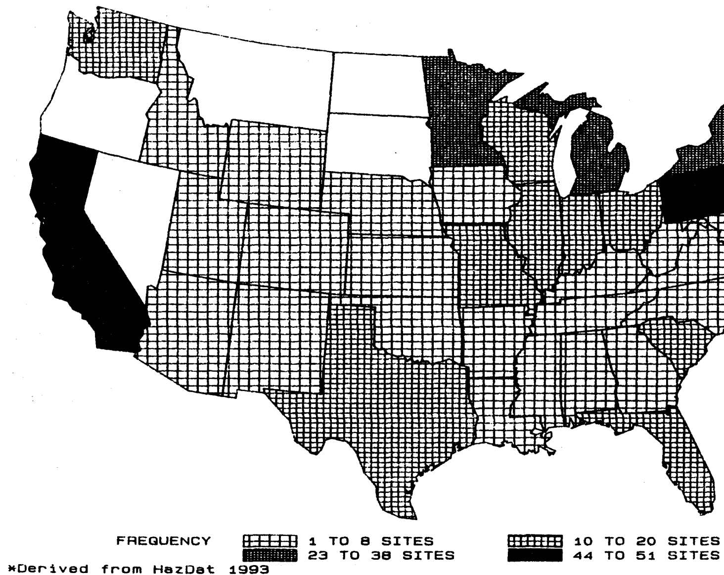
FIGURE 5-1. FREQUENCY OF NPL SITES WITH 1,1-DICHLOROETHENE CONTAMINATION *
