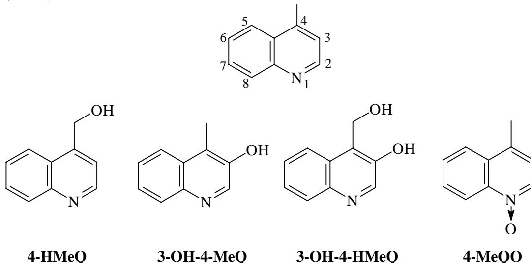
Figure 1. Metabolites of 4-methylquinoline identified from in vitro studies (Saeki et al. , 1996).
