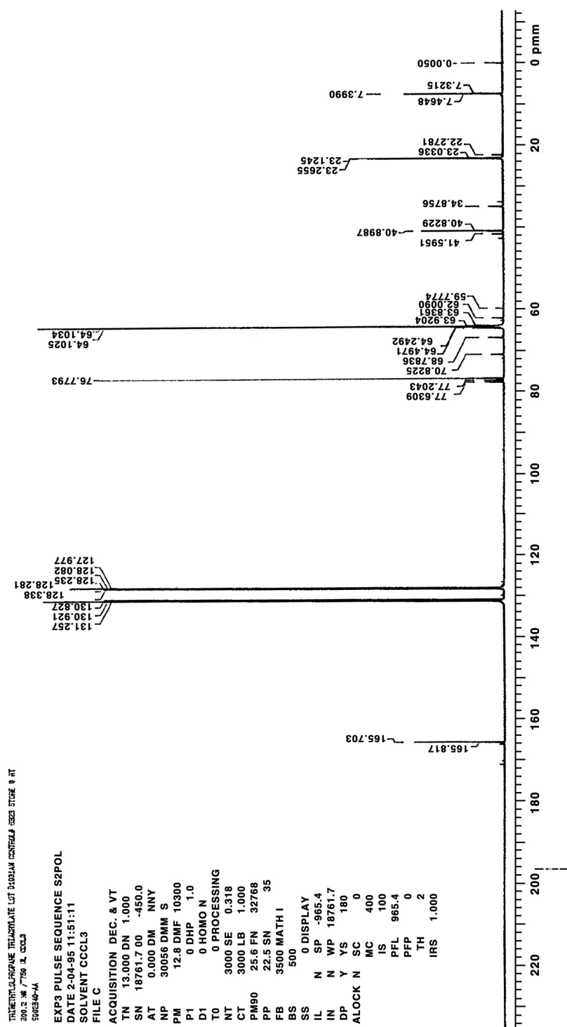
FIGURE H3 ^{13}\text{C} Nuclear Magnetic Resonance Spectrum of Trimethylolpropane Triacrylate
