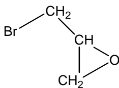
Figure 1-5. Structure of 3-bromo-1,2-propane epoxide
