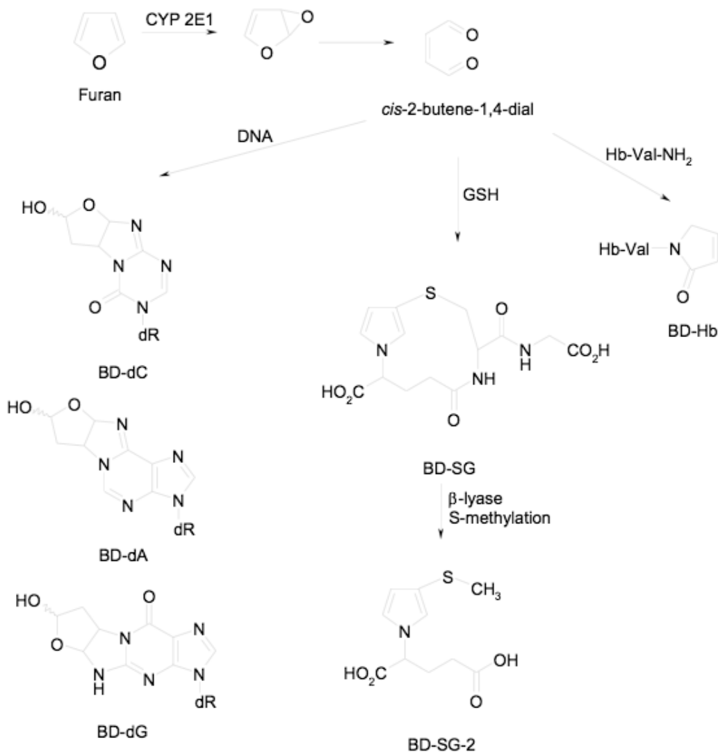
Figure 1. Oxidative metabolism of furan and formation of potential biomarkers.
